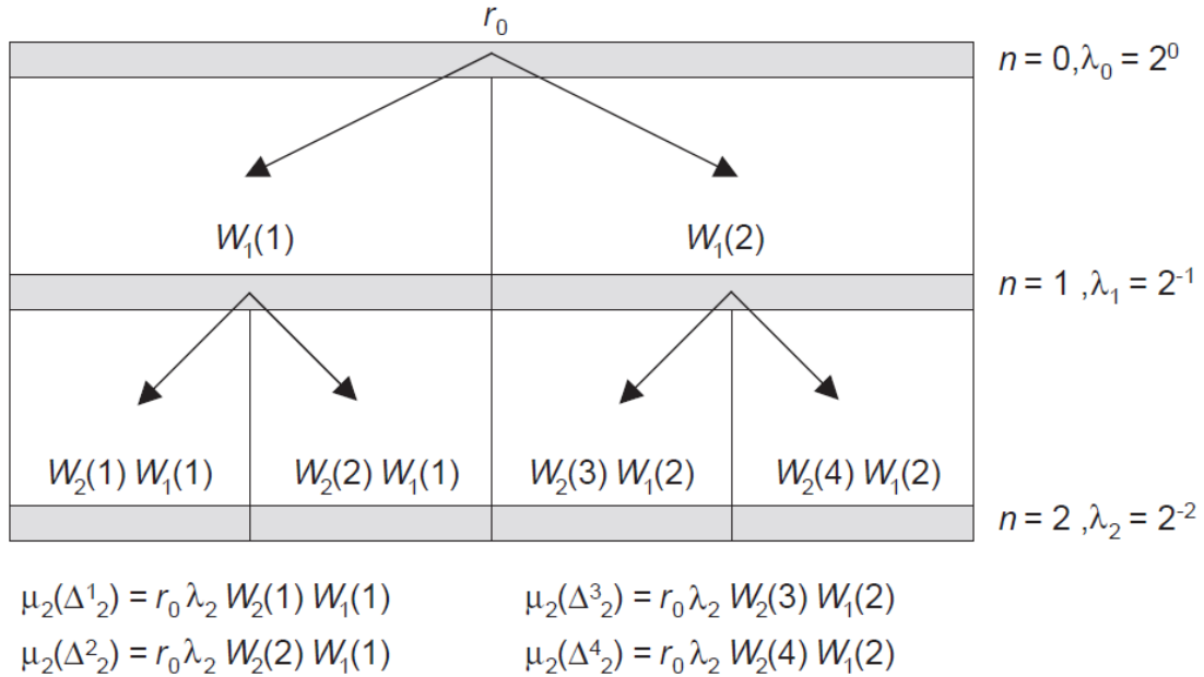
Figure 16: Framework of canonical random cascade model with branching number b = 2 and cascade generator W for scales n = 0, 1 and 2 . r_0 denotes rainfall amount at scale 0 , which in many applications corresponds to daily rainfall (extracted from Molnar and Burlando, 2005).
