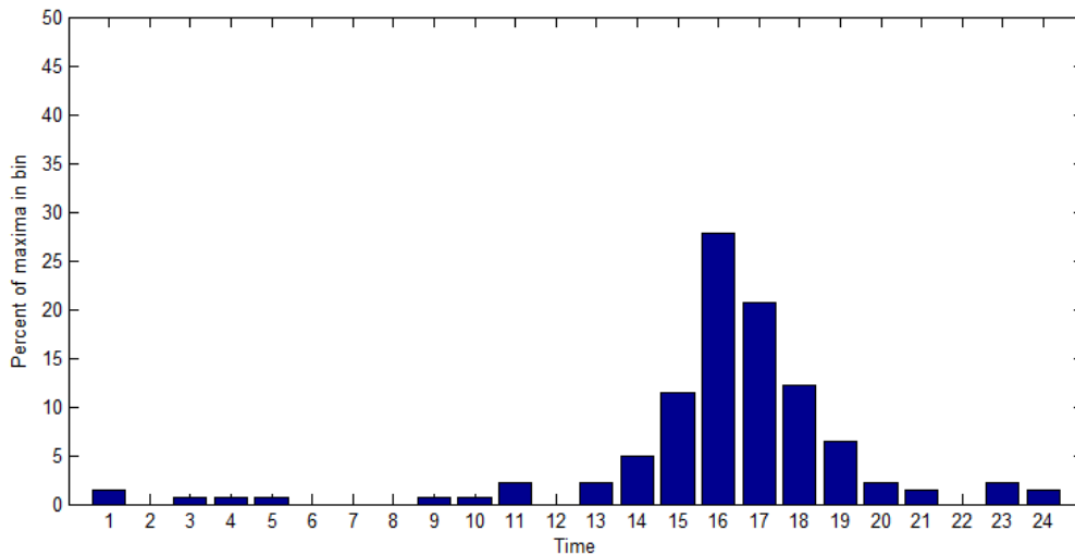
Figure 12: Percentage of stations with intensity maxima against time of the day for summer
