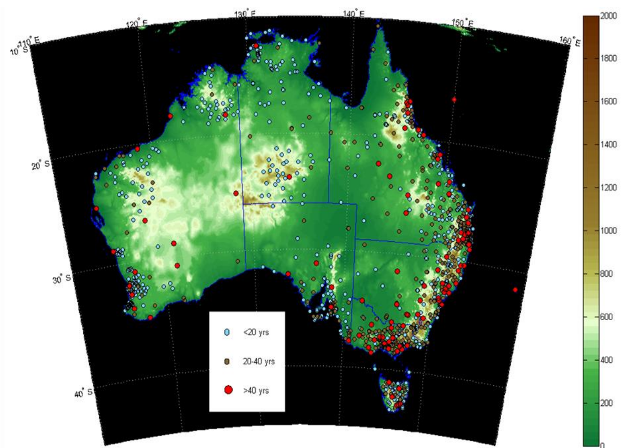
Figure 1: Spatial coverage and record length of the Australian continuous rainfall record.
