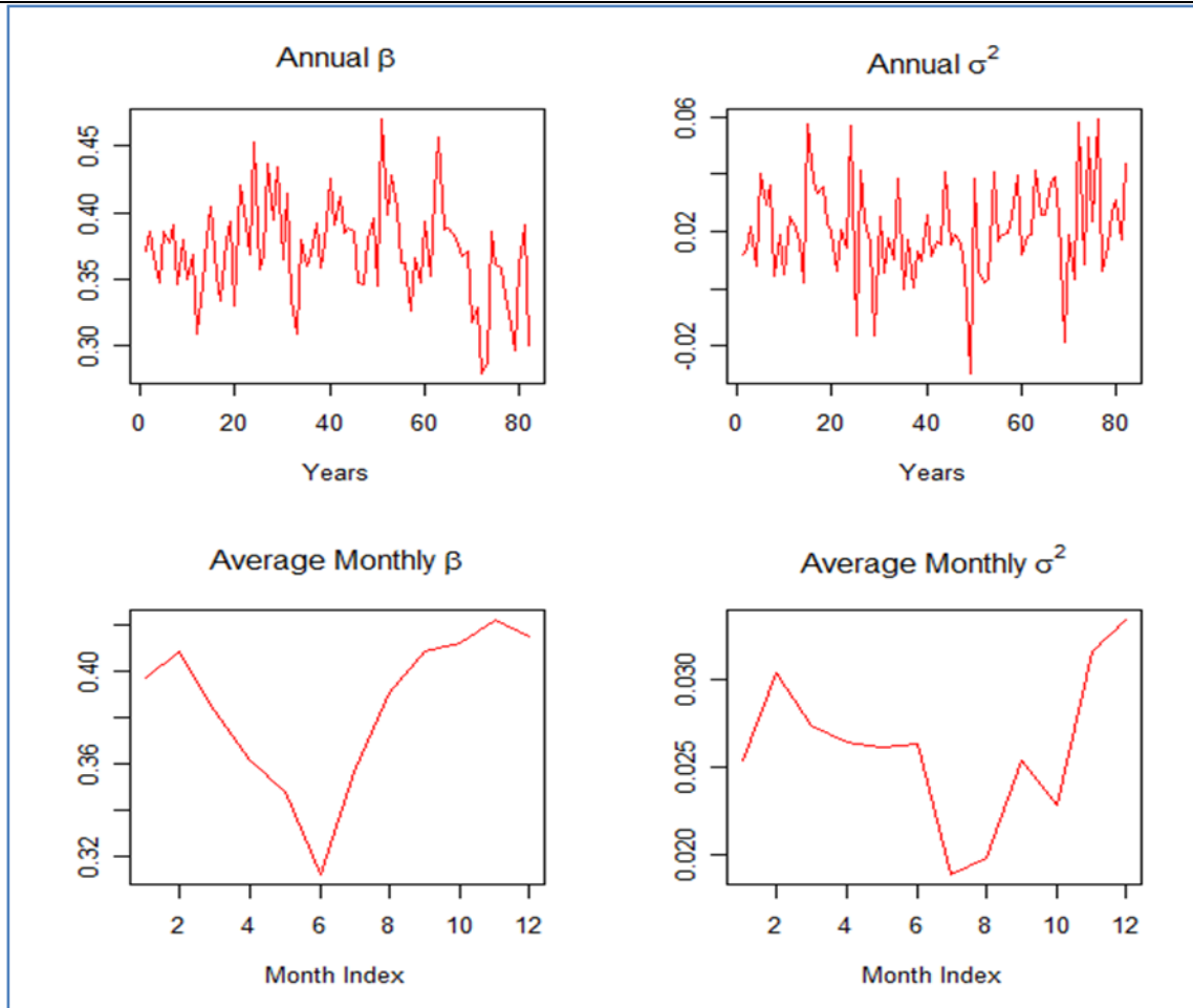
Figure 5: Parameters of the canonical model estimated on an annual and monthly basis. Note that the use of a single set of parameters fitted to the entire rainfall record therefore does not account for inter annual and seasonal fluctuations.
