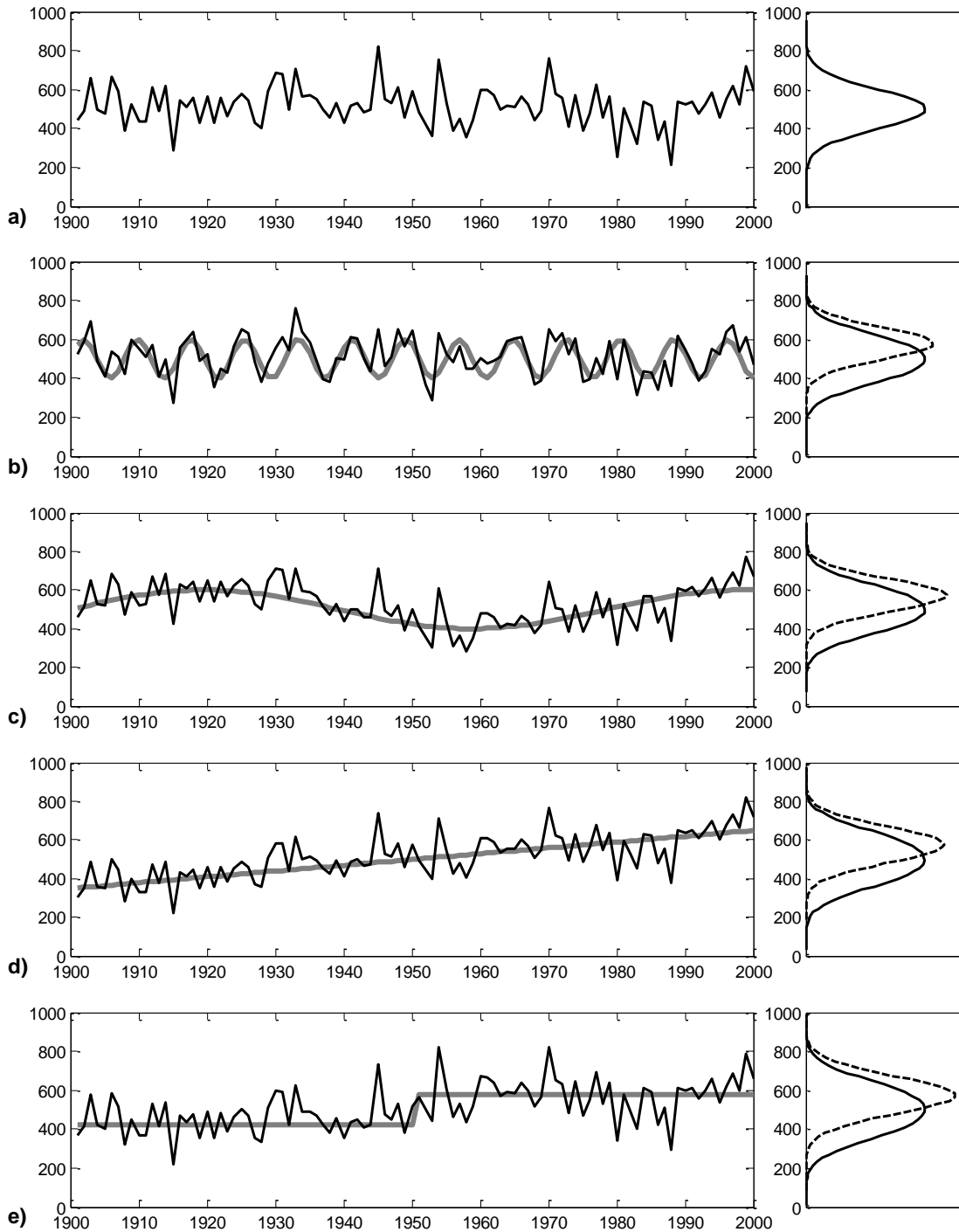
Figure 1: The implications of different forms of non-stationarity in evaluating future flood risk. The left panels represent a randomly generated sample of length 100, and the right panels represent the underlying population distribution, including the unconditional sample distribution (black solid line) and a conditional distribution based on only a subset of the data (black dashed line). Panel (a) comprises a normally distributed stationary time series, with the remaining panels being the summation of the data in (a) (thin black line) and an underlying non-stationarity component (thick gray line). Specifically: (b) represents cyclical variability with a period much shorter than the period of record; (c) represents cyclical variability with period of similar length to the period of record; (d) represents a long-term trend; and (e) represents a step change.
