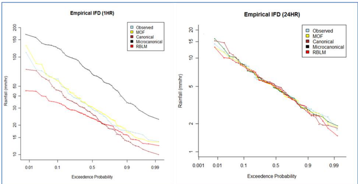
Figure 6: 1 and 24HR Empirical IFD curves for observed rainfall and disaggregated rainfall by the models.
