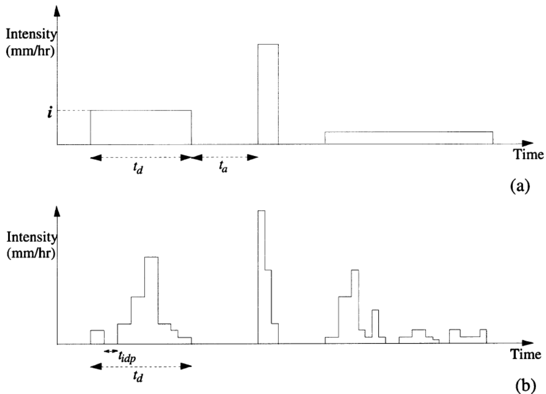
Figure 14: The Disaggregated Rectangular Intensity Pulse model (extracted from Heneker et al , 2001).
