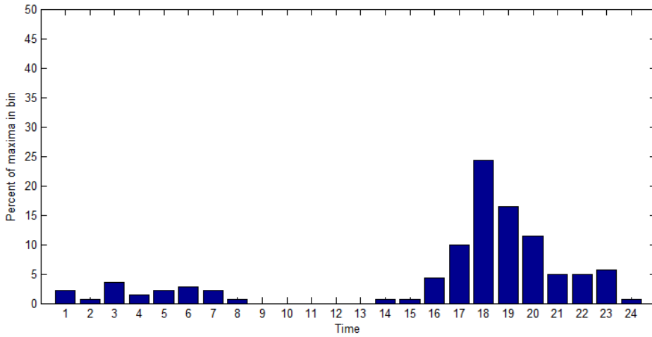
Figure 9: Percentage of stations with frequency maxima against time of the day for summer.
