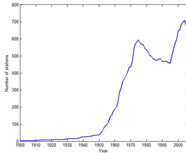
Figure 2: Number of Australia-wide continuous rainfall records against year of record.
