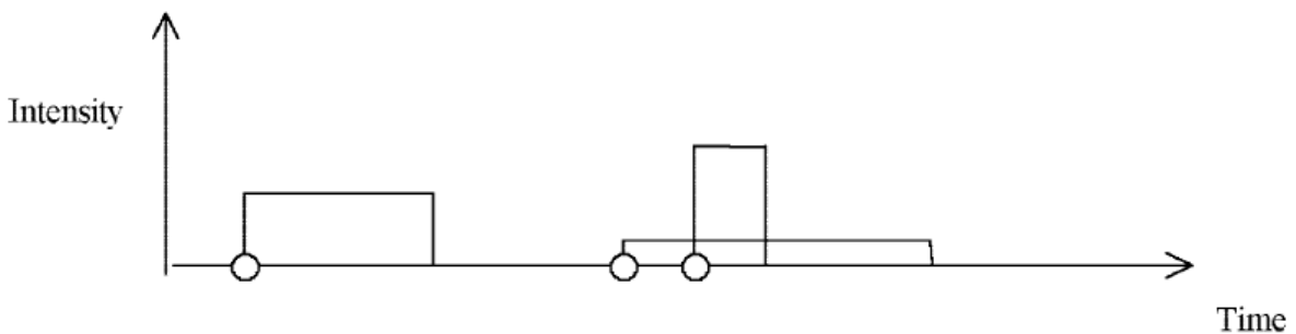
Figure 15: (a) Schematic for Poisson cluster point-process models; (b) schematic for the rectangular pulse model (extracted from Onof et al , 2000).
