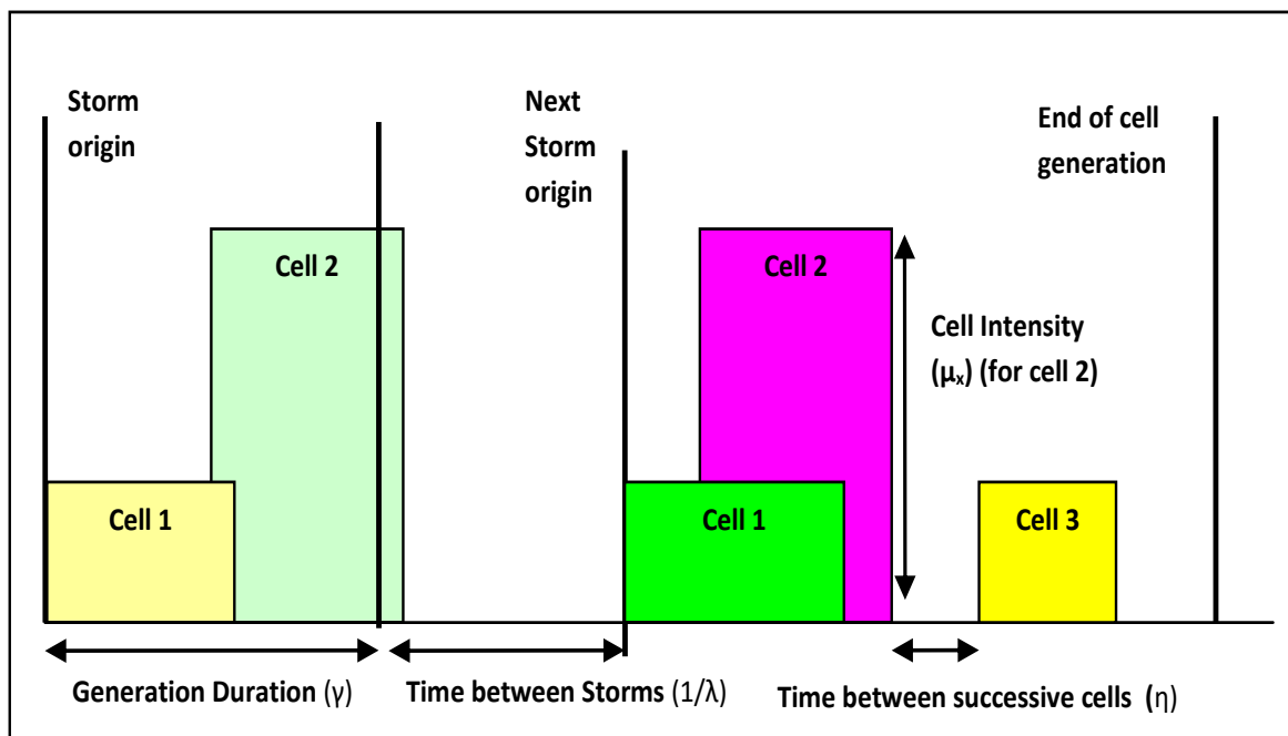
Figure 3: Schematic showing RBLM process. Storm arrivals follow Poisson process with mean of 1/\lambda , with generation duration of each storm exponentially distributed with mean 1/\gamma . First cell is fixed to occur at storm origin while later cells within a storm arrive by a second Poisson process with expected value of \beta . Duration of each cell is exponentially distributed with mean of 1/\eta . Each cell's intensity is exponentially distributed with a mean of \mu_x .
