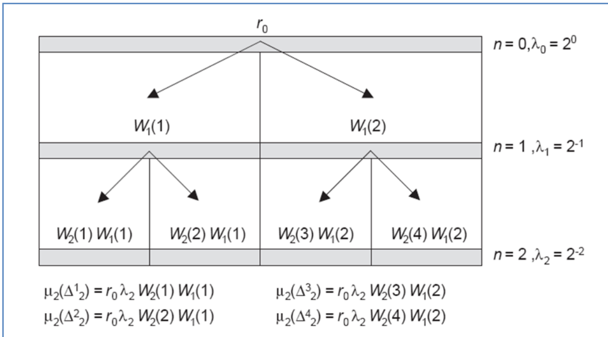
Figure 1: Framework of canonical RMC with branching number b = 2 and cascade generator W for scales n = 0, 1 , and 2 . r_0 denotes , rainfall amount at scale 0, (i.e. daily rainfall) (Molnar and Burlando, 2005)
