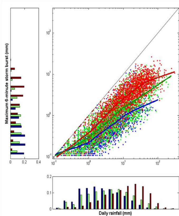
Figure 3: Maximum 6-minute storm burst against daily rainfall for each wet day, for Darwin (red), Sydney (green) and Hobart (blue), plotted on a logarithmic scale. Mean response estimated using a LOESS smoother fit to the log-transformed data. Plot includes marginal histogram of 6-minute (left panel) and daily (bottom panel) rainfall, and joint scatterplot (centre panel)
