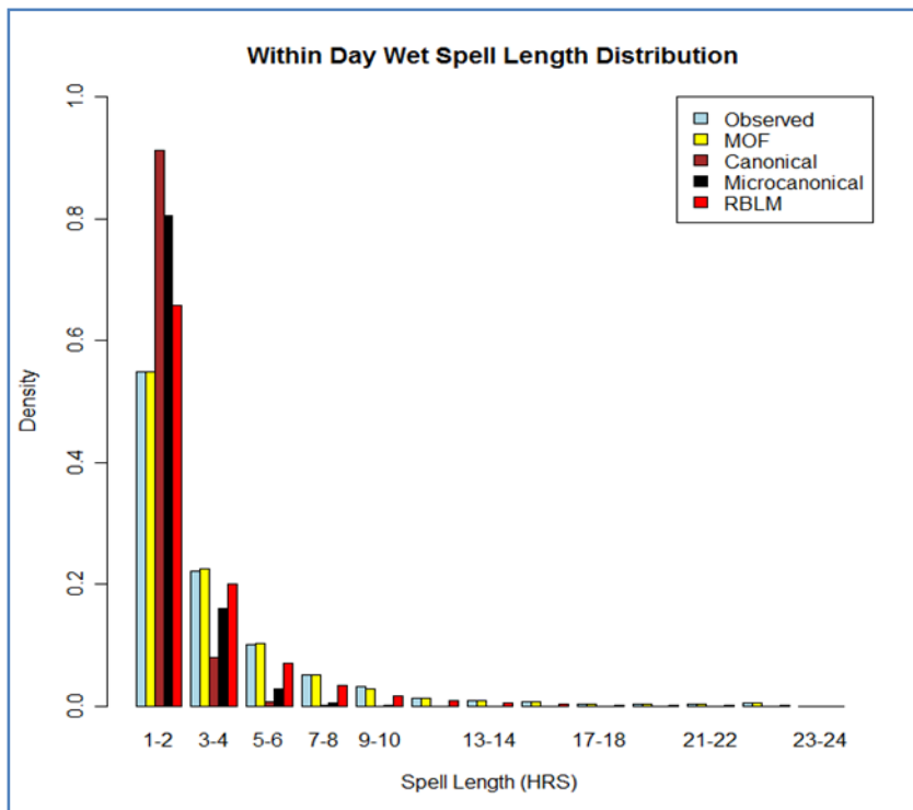
Figure 7: Within Day Wet Spell Distribution for disaggregation models compared to observed wet spells.
