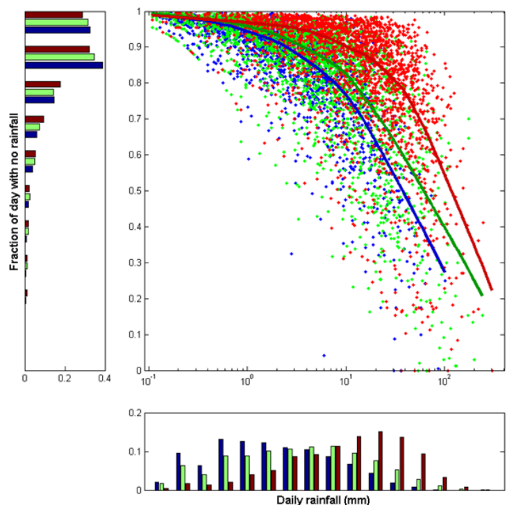
Figure 4: as for Figure 3, but with fraction of wet day with no rainfall plotted against daily rainfall amount.
