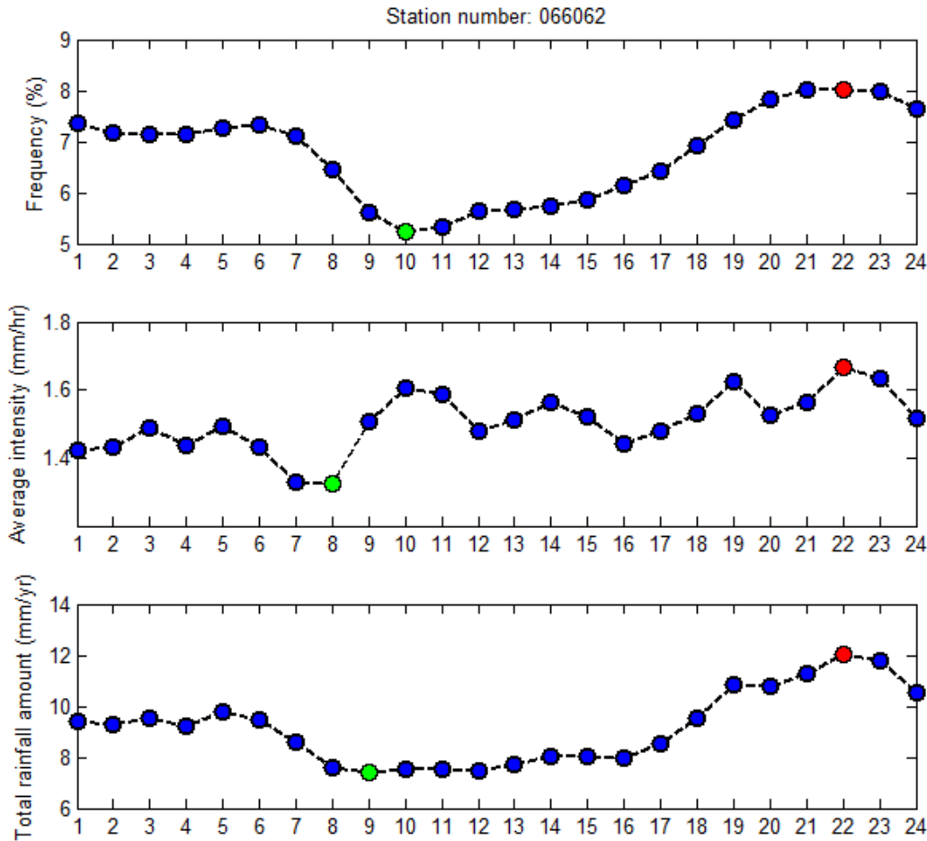
Figure 6: The diurnal cycle of frequency, average intensity and total rainfall amount plotted against time of day for Sydney Observatory Hill during the summer. The hourly data was smoothed using a three-point smoother, with the timing of the minima and maxima represented by green and red dots, respectively.
