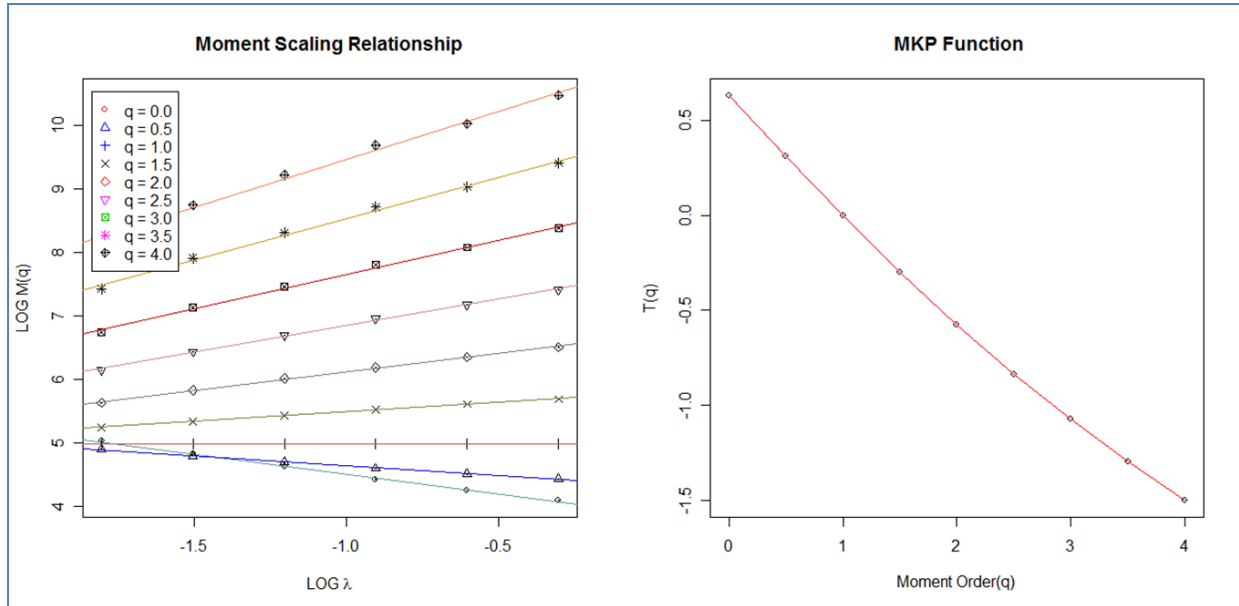
Figure 2: Moment Scaling Relationships (left) and the MKP function (right) for observed data at the Observatory Hill Gauge, Sydney. Slope of lines on plot of Moment Scaling Relationships shows rate of divergence/ convergence of moments with scale.
