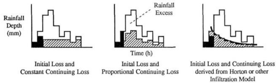
Figure 2-3 Commonly used loss models as described by O’Loughlin et al. (1996).
