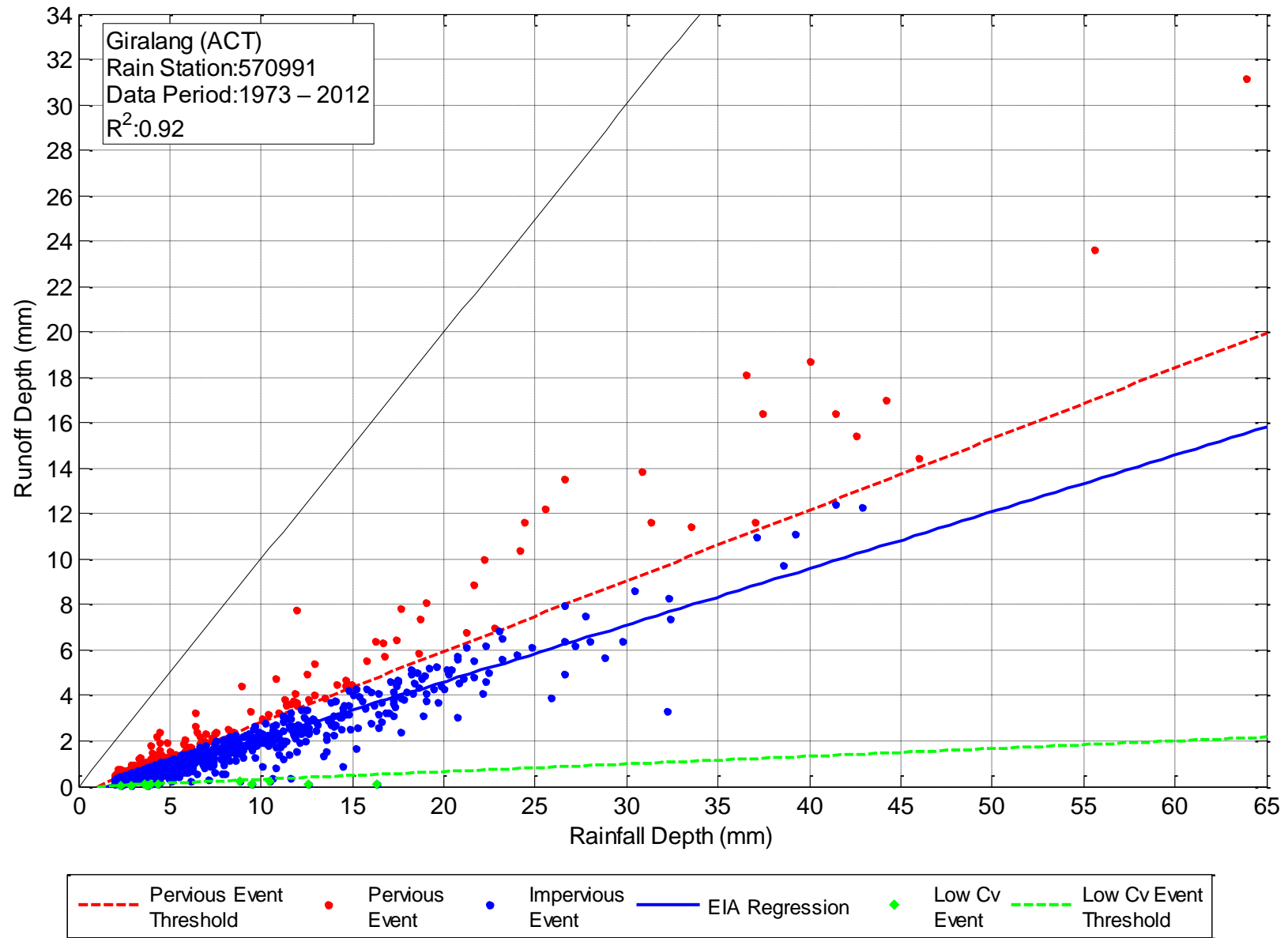
Figure C-7. Regression of Rainfall and Runoff – Giralang (ACT), Rain Gauge 570991, Data Period 1973 - 2012
