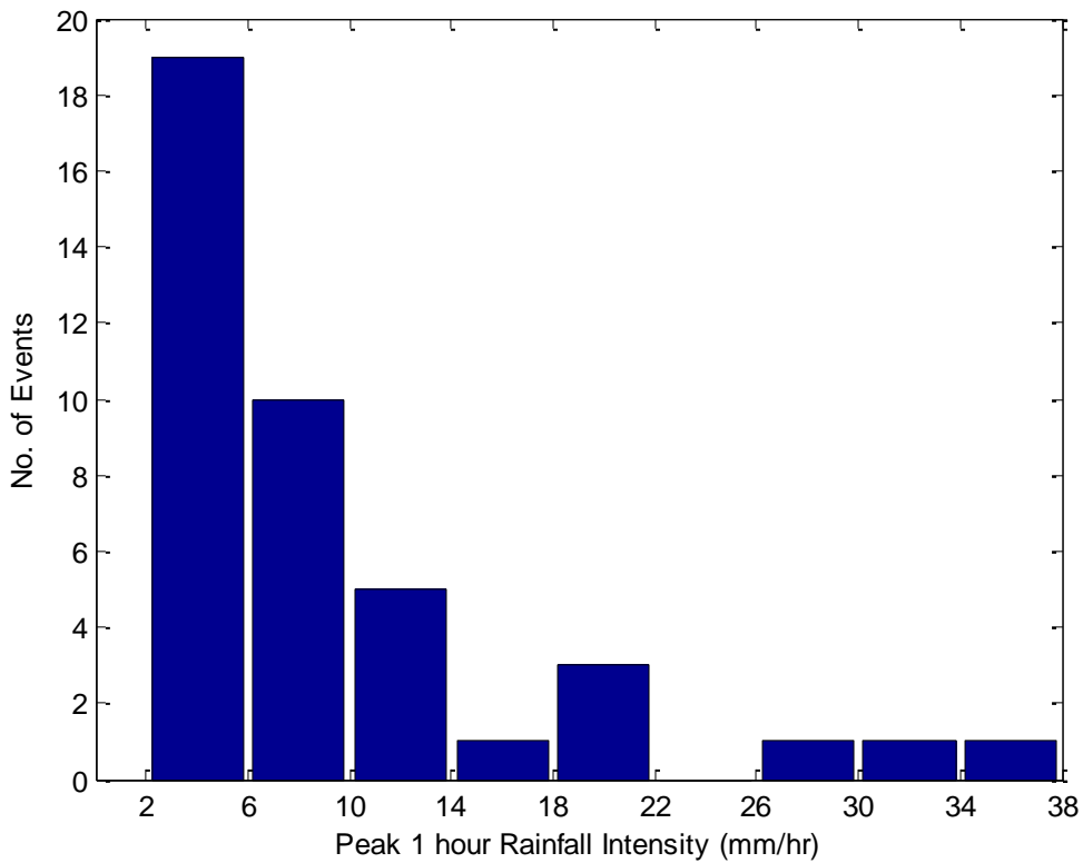
Figure 8-9. Giralang - 1 hour Rainfall Intensity Histogram
