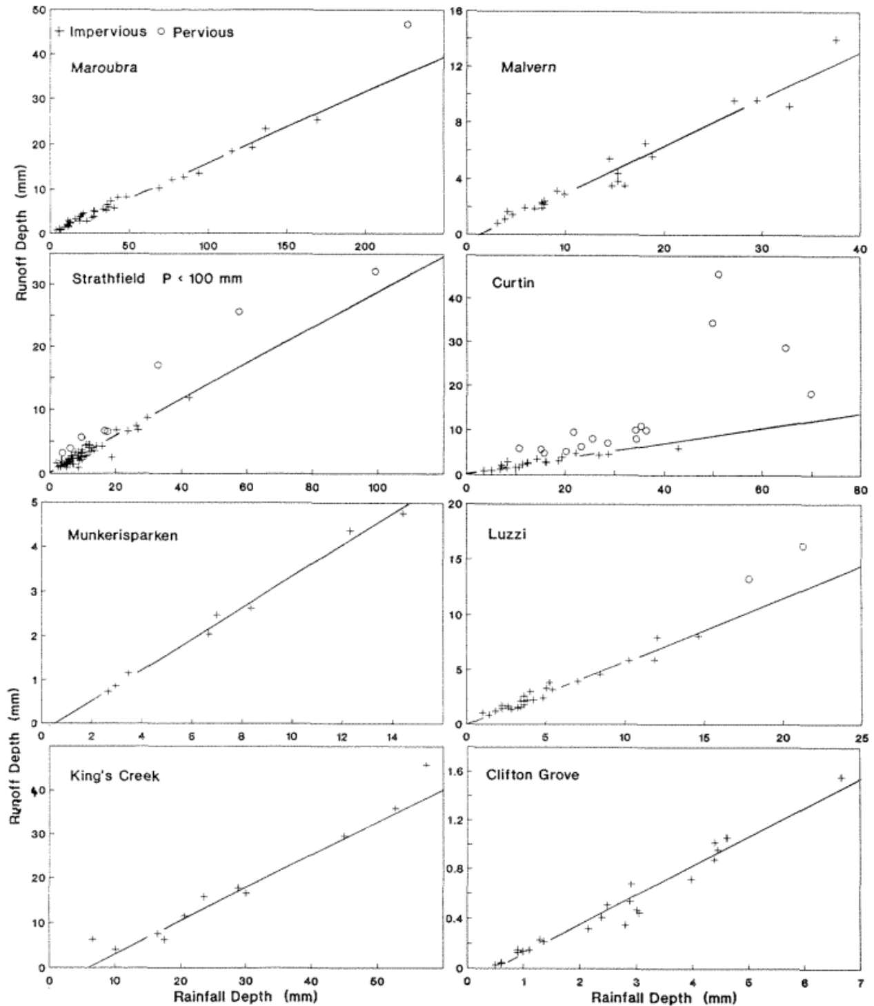
Figure 2-1 Rainfall vs Streamflow Depths For A Select Group Of Catchments (Boyd, Bufile & Knee, 1993)
