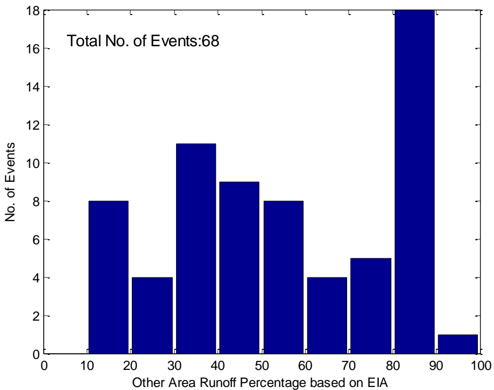
Figure 8-8. Ithaca Creek (QLD) - Histogram of Identified Storm Events – Volume of Runoff from Other Area relative to total runoff
