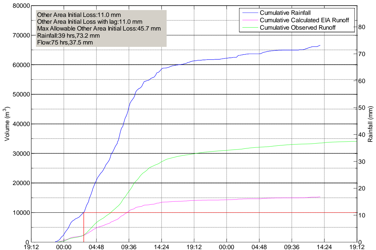
Figure 7-3 Example estimation of Other Area Initial Loss using cumulative volumes for an historical event in the Giralang Catchment.
