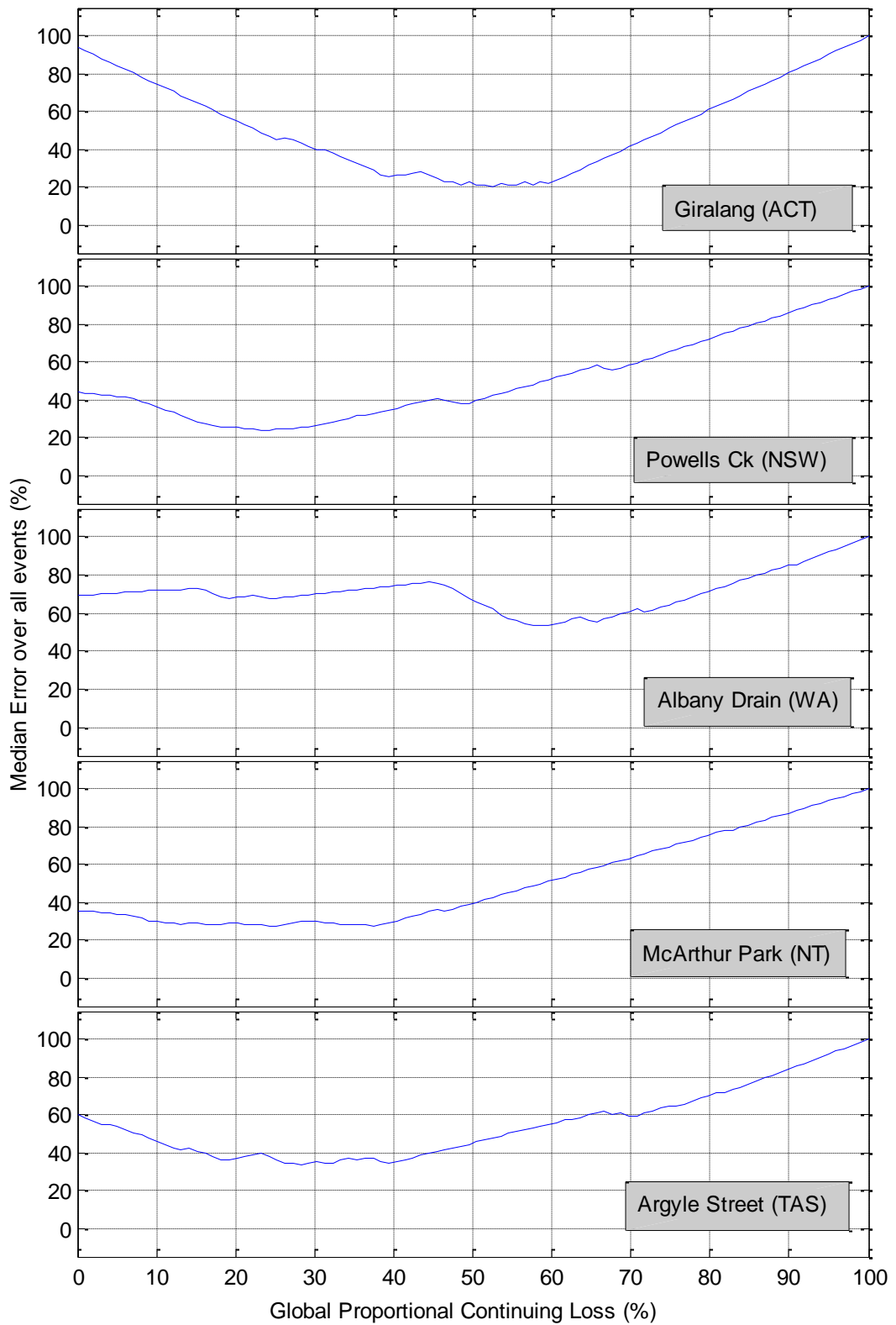
Figure 9-10 Median Error when optimising over all events for the range of Proportional Continuing Loss Values
