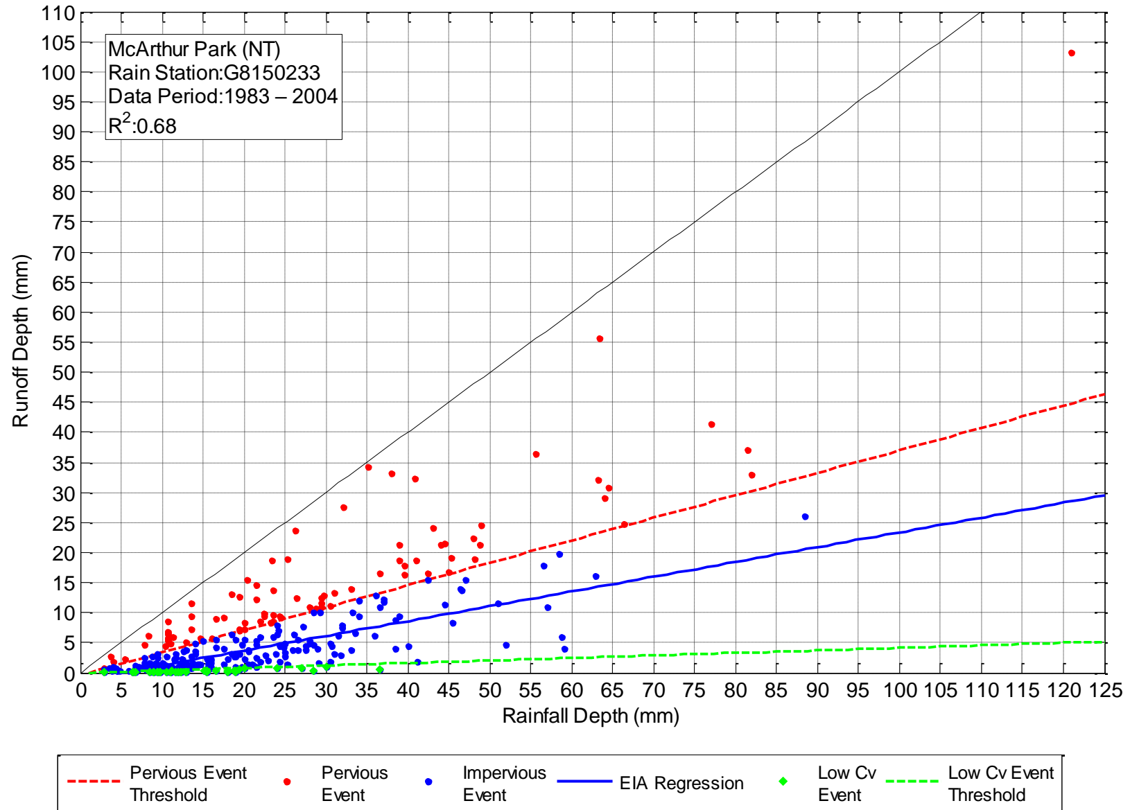
Figure C-11. Regression of Rainfall and Runoff – McArthur Park (NT)
