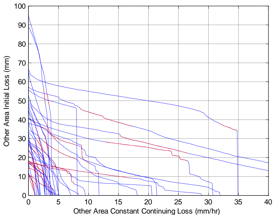
Figure 9-4. Contour Plot of Initial Loss & Constant Continuing Loss - Giralang (ACT)
