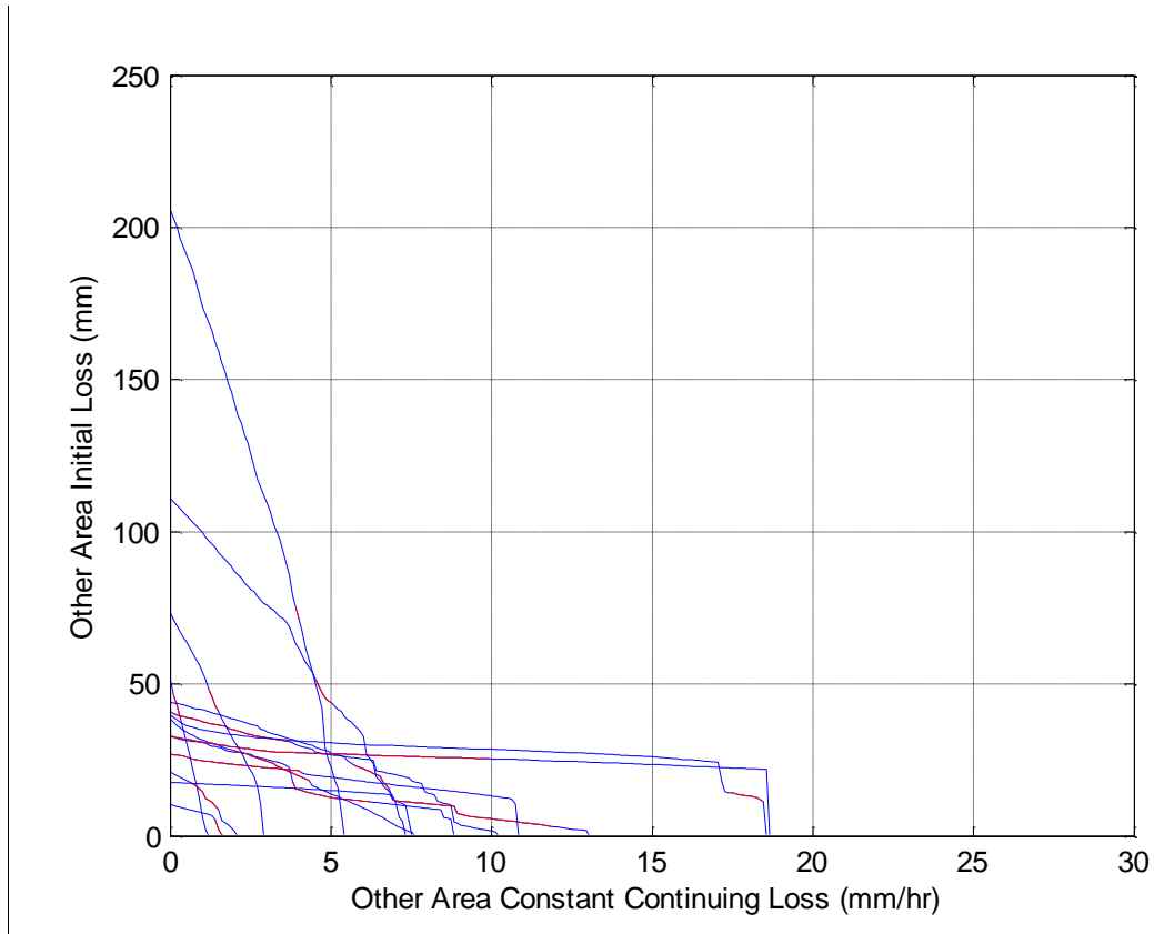
Figure 9-5. Contour Plot of Initial Loss & Constant Continuing Loss – PowellsCk (NSW)
