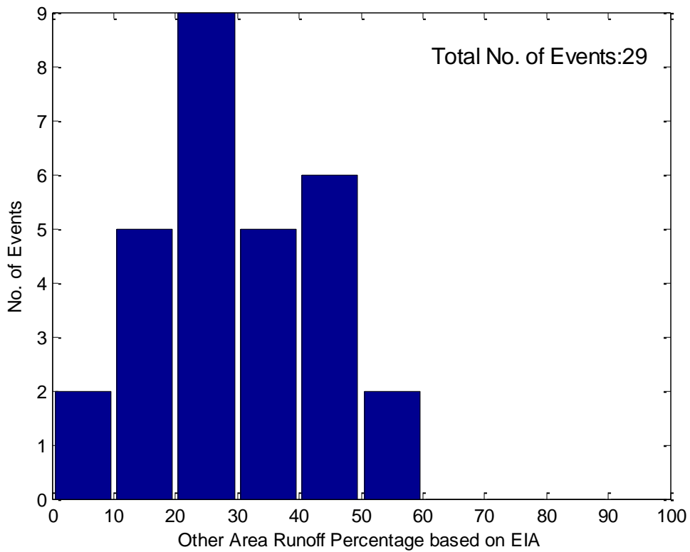
Figure 8-7. Powells Creek (NSW) - Histogram of Identified Storm Events – Volume of Runoff from Other Area relative to total runoff
