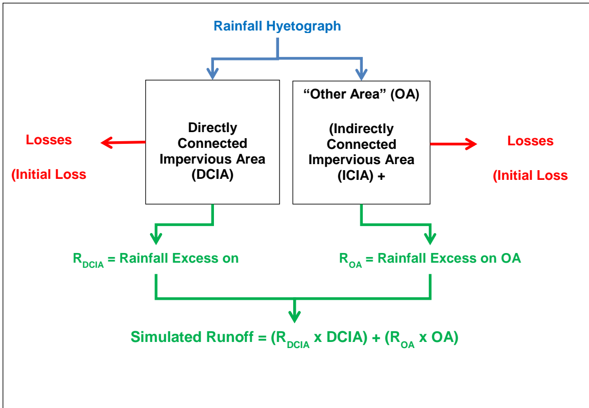
Figure 7-1 Methodology to determine losses based on volumetric analysis of historical storm events
