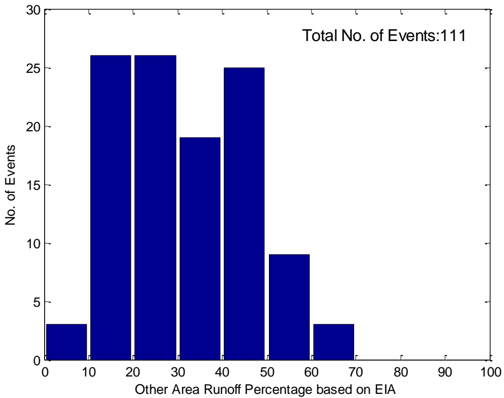
Figure 8-1. Giralang (ACT) - Histogram of Identified Storm Events – Volume of Runoff from Other Area relative to total runoff
