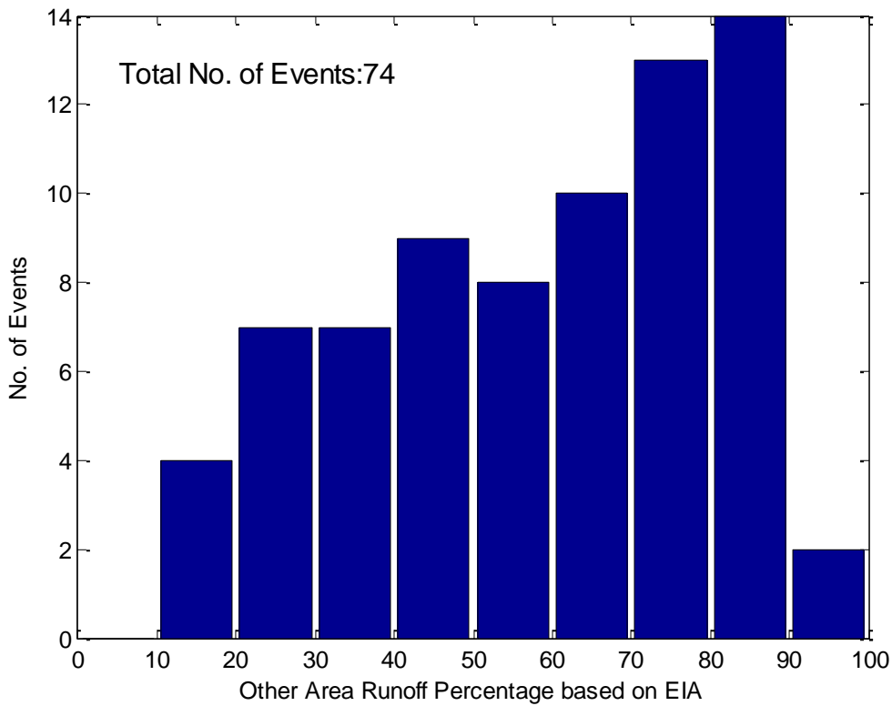
Figure 8-3. Argyle Street (TAS) - Histogram of Identified Storm Events – Volume of Runoff from Other Area relative to total runoff
