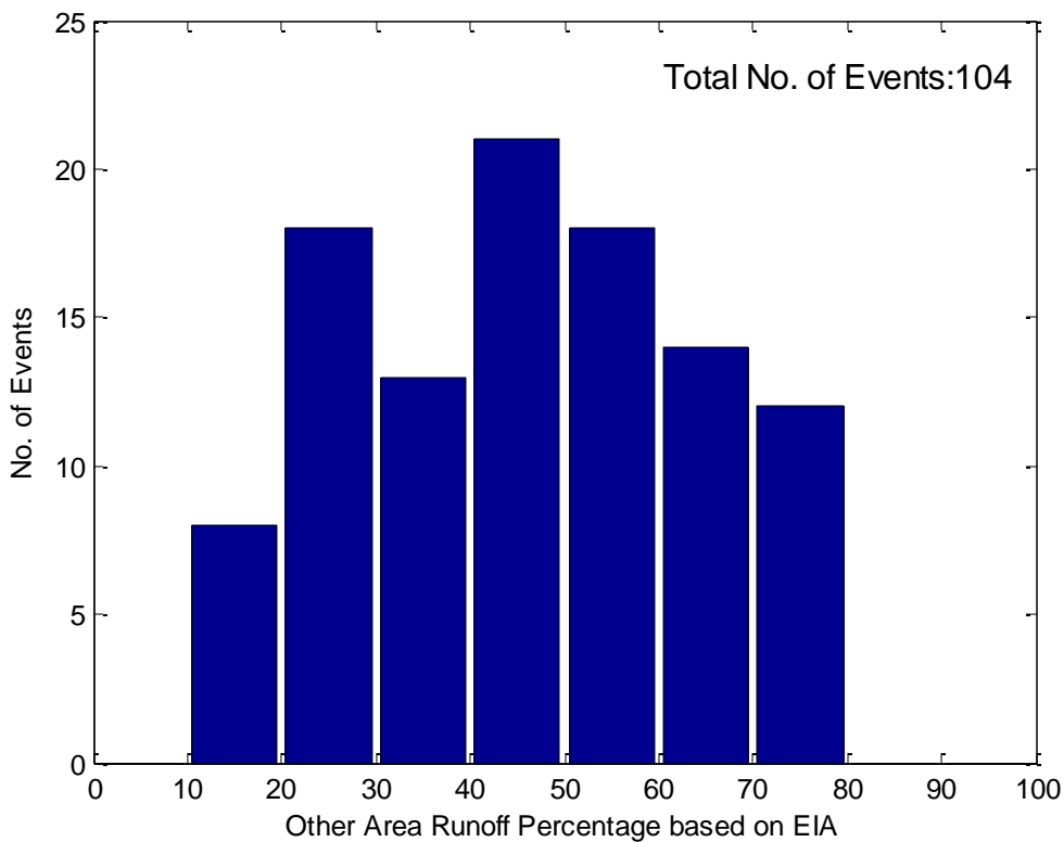
Figure 8-4. McArthur Park (NT) - Histogram of Identified Storm Events – Volume of Runoff from Other Area relative to total runoff
