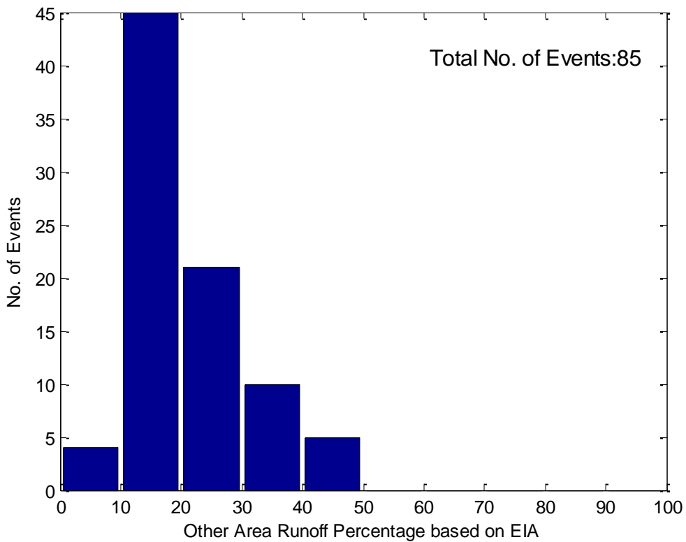
Figure 8-2. Albany Drain (WA) - Histogram of Identified Storm Events – Volume of Runoff from Other Area relative to total runoff
