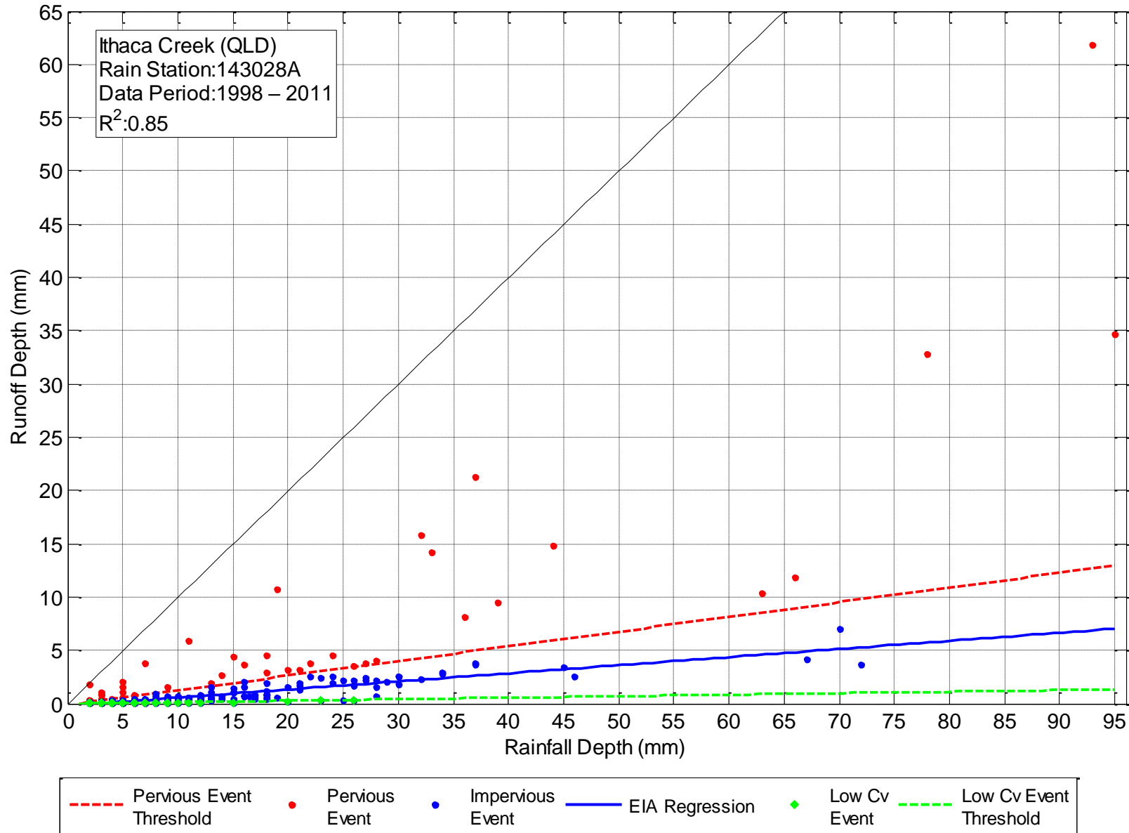
Figure C-9. Regression of Rainfall and Runoff – Ithaca Creek (QLD)
