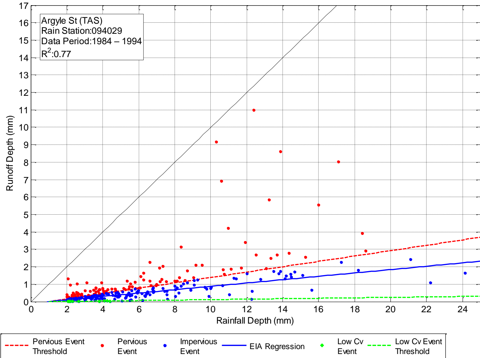
Figure C-2. Regression of Rainfall and Runoff – Argyle Street (TAS)
