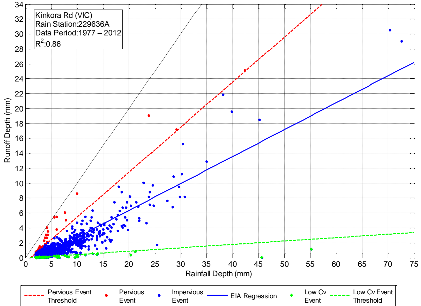
Figure C-10. Regression of Rainfall and Runoff – Kinkora Road (VIC)
