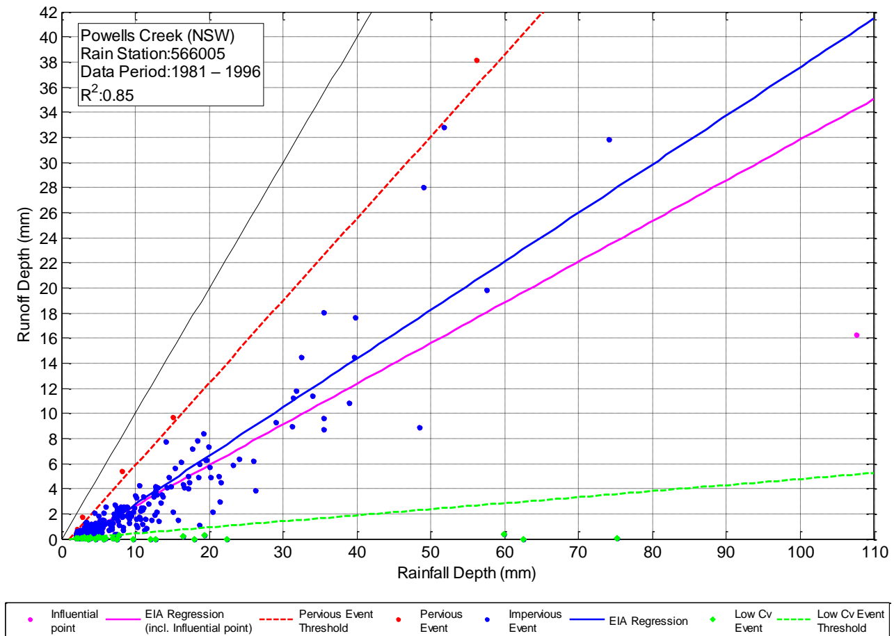
Figure 6-3 Impact of an influential data point on the regression analysis for the Powells Creek Catchment
