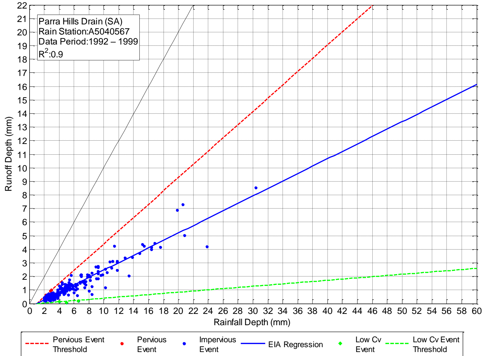
Figure C-12. Regression of Rainfall and Runoff – Para Hills Drain (SA)
