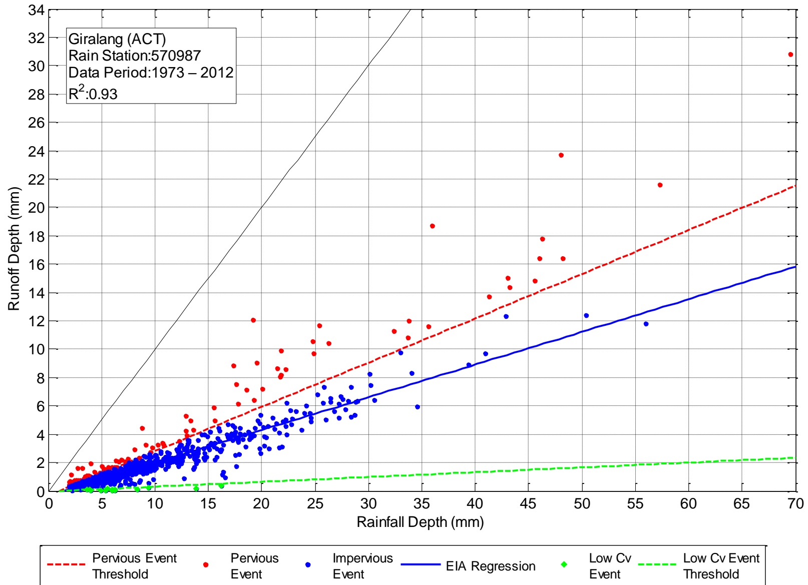
Figure C-4. Regression of Rainfall and Runoff – Giralang (ACT), Rain Gauge 570987, Data Period 1973 - 2012
