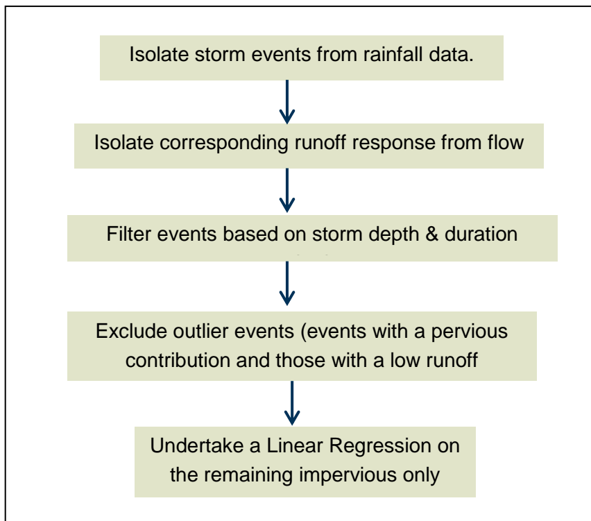
Figure 5-1 Methodology for estimating EIA using rainfall and streamflow data
