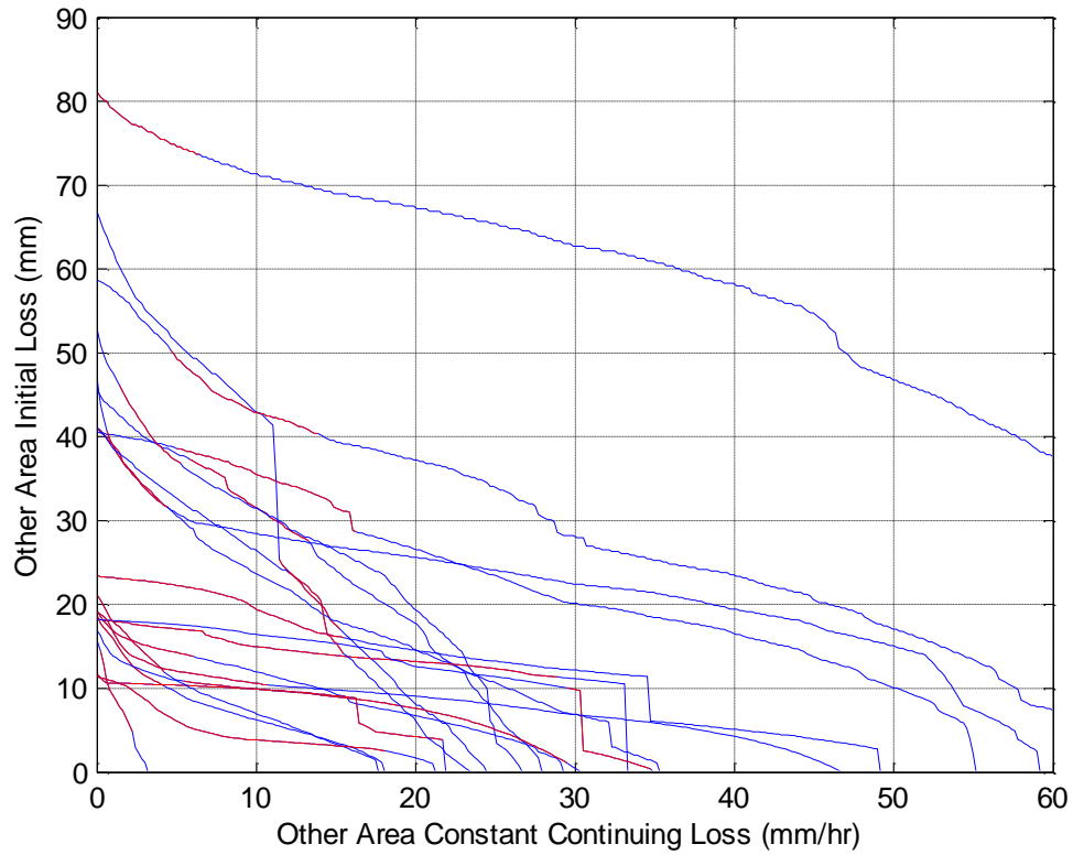
Figure 9-7 Contour Plot of Initial Loss & Constant Continuing Loss – McArthur Park (NT)
