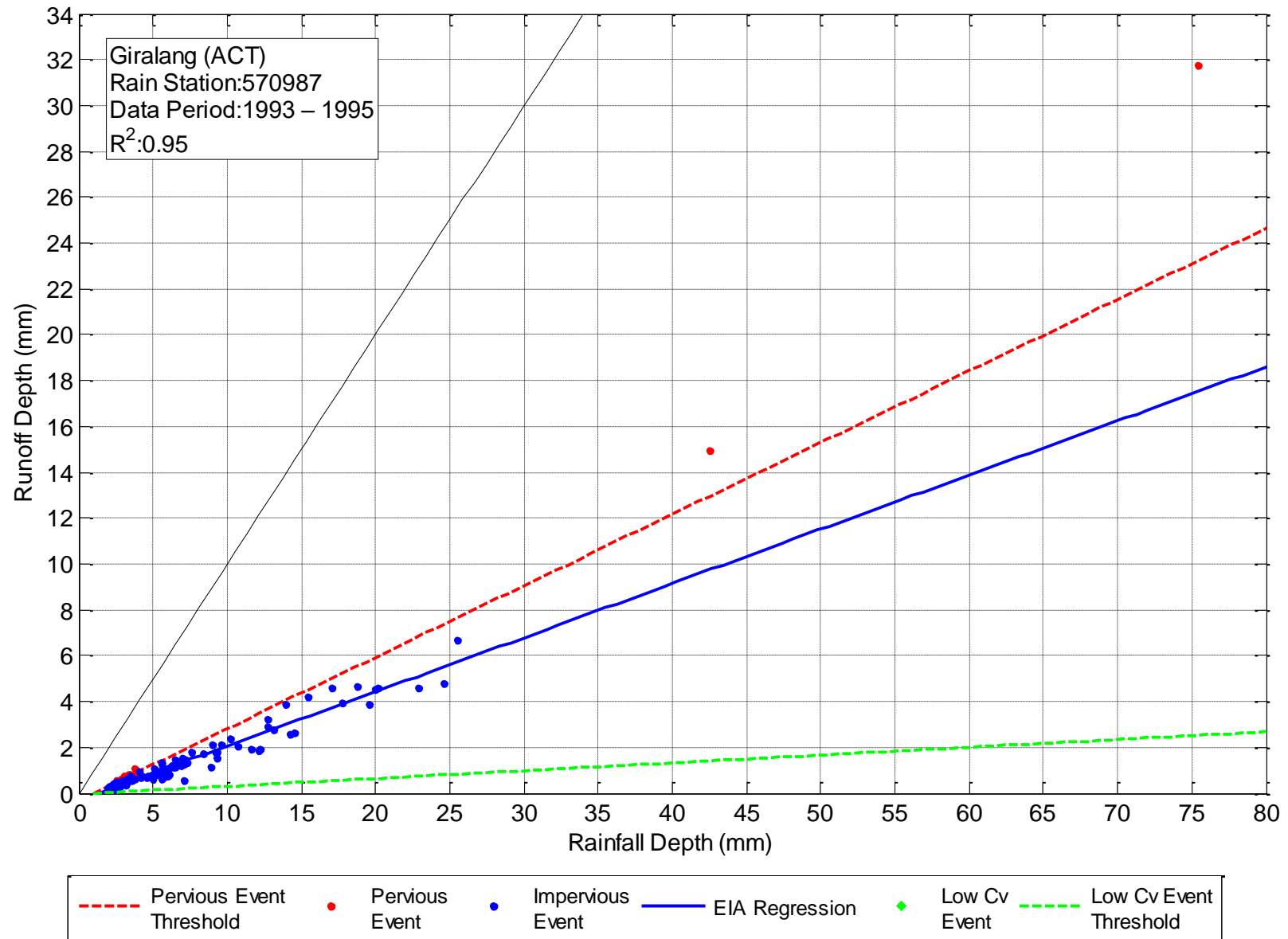
Figure C-3. Regression of Rainfall and Runoff – Giralang (ACT), Rain Gauge 570987, Data Period 1993 - 1995
