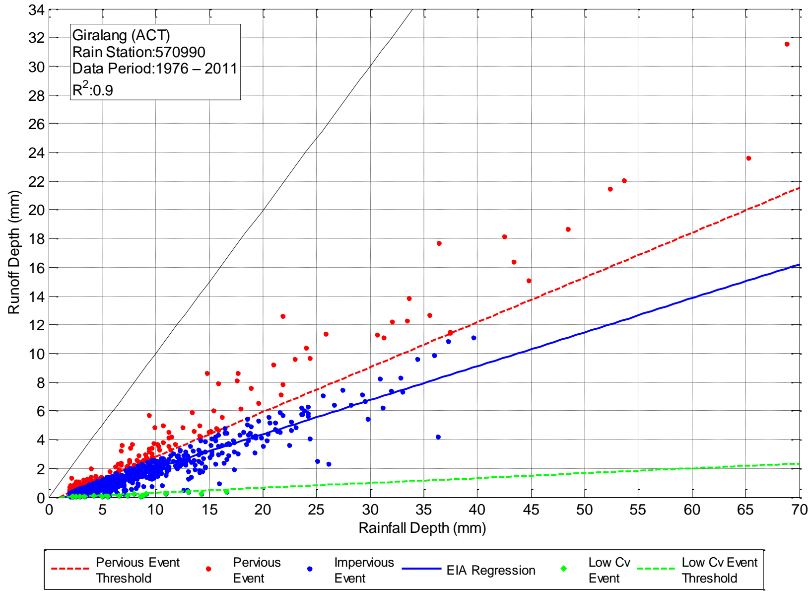
Figure C-5. Regression of Rainfall and Runoff – Giralang (ACT), Rain Gauge 570990, Data Period 1976 - 2011
