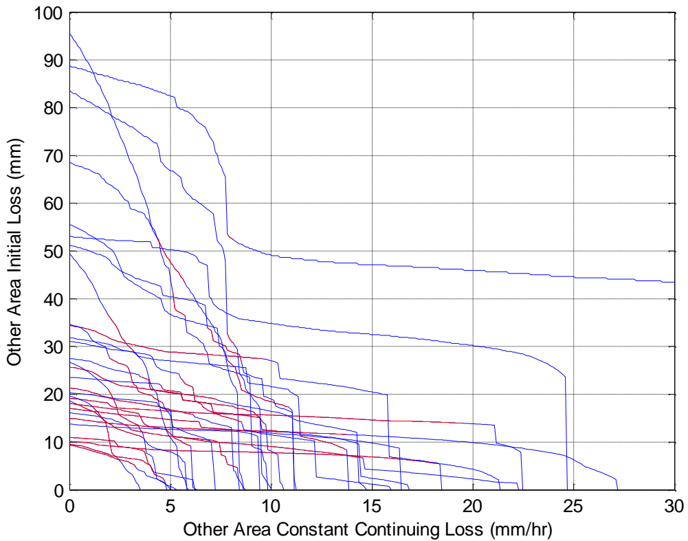
Figure 9-6. Contour Plot of Initial Loss & Constant Continuing Loss – Albany Drain (WA)
