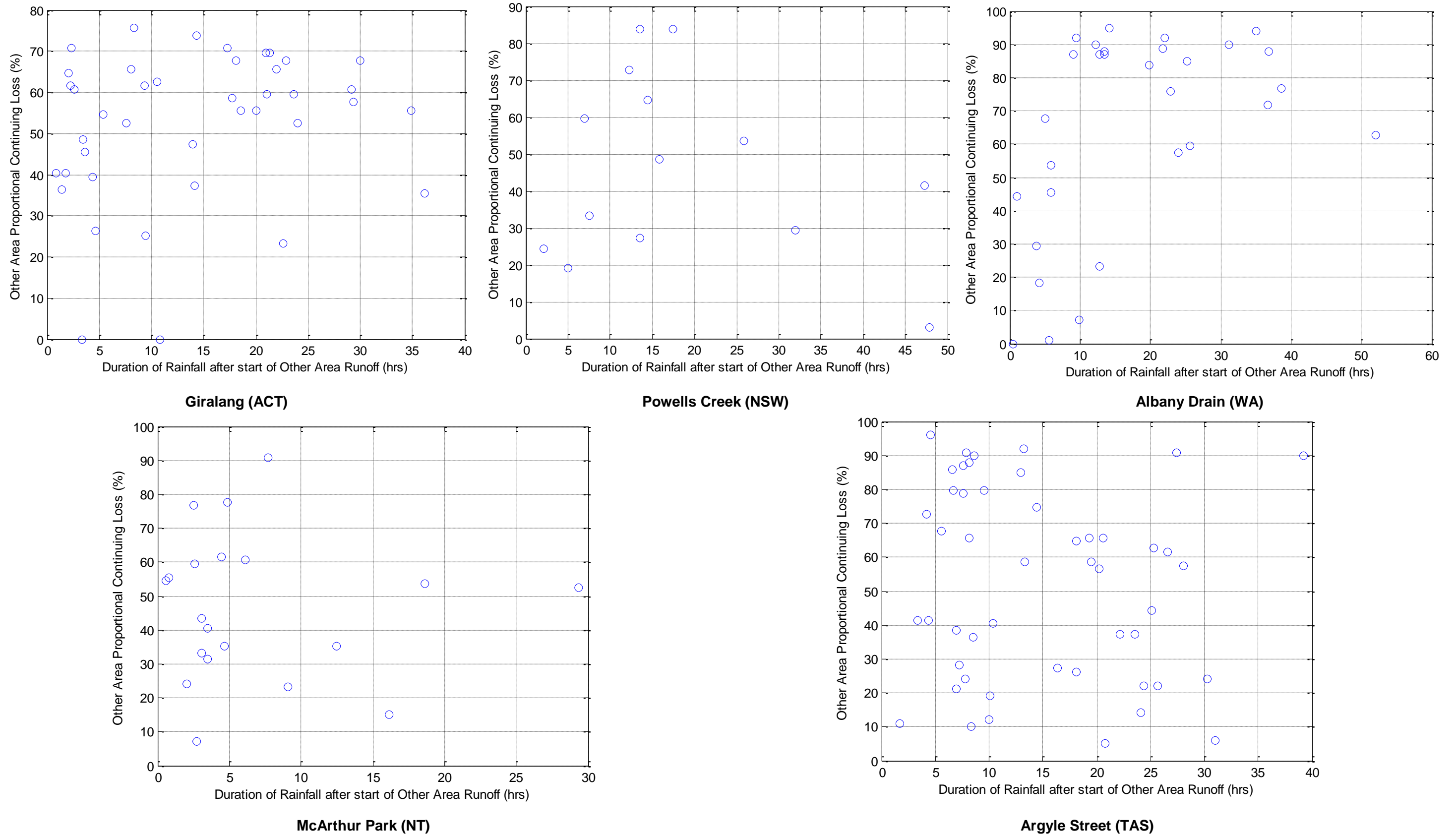
Figure E-6. Correlation Analysis – Other Area Proportional Continuing Loss vs Duration after Other Area Runoff
