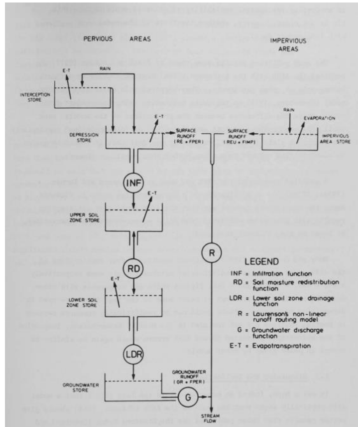
Figure 2-4 The model structure of the Australian Representative Basins model based on the work of Chapman (1968). Diagram obtained from Black and Aitken (1977) and Mein & McMahon (1982).
