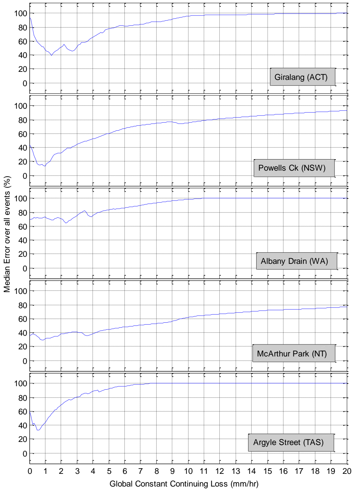
Figure 9-3 Median Error when optimising over all events for the range of Constant Continuing Loss Values
