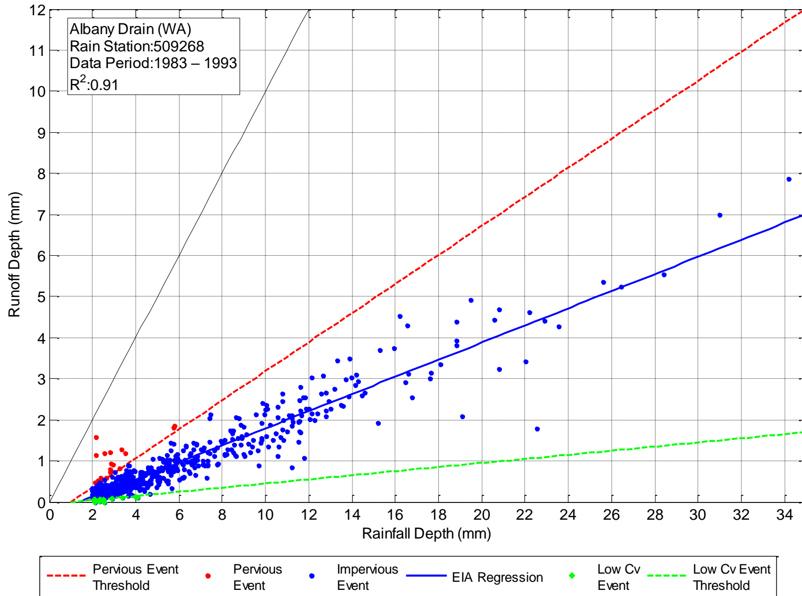
Figure C-1. Regression of Rainfall and Runoff – Albany Drain (WA)
