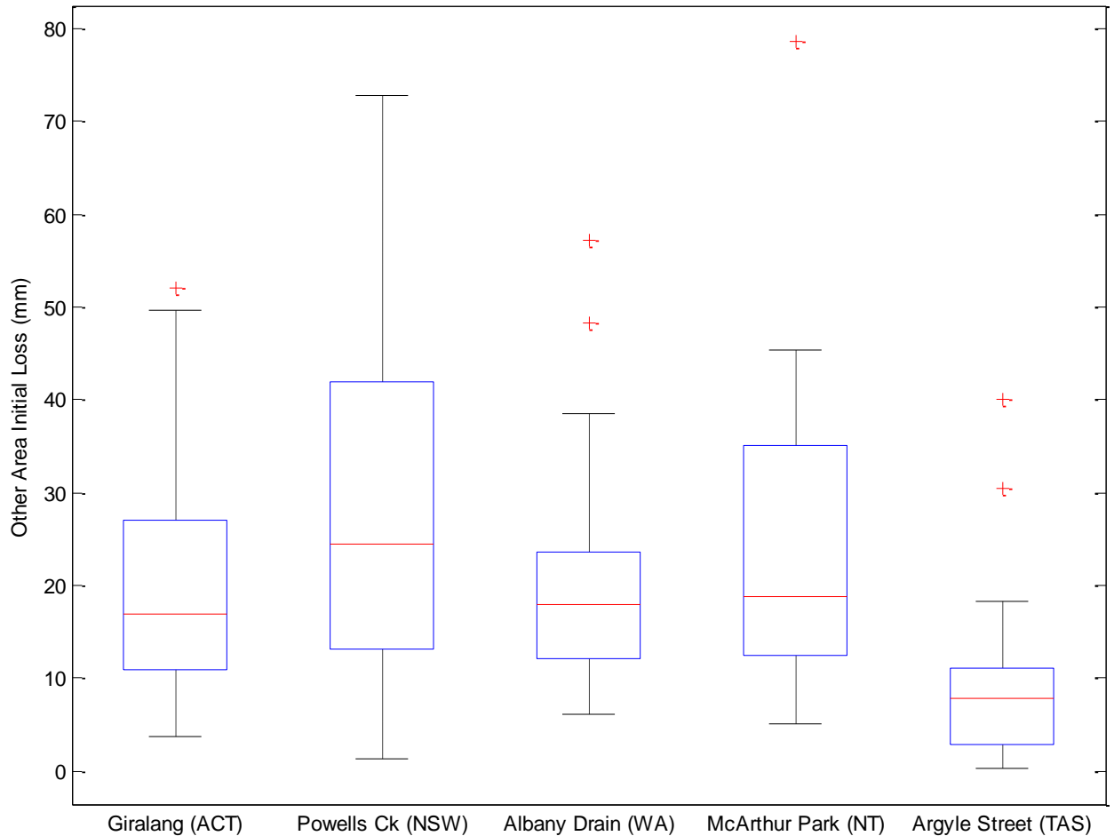
Figure 9-1 Boxplot of Other Area Initial Loss Estimates (Giralang: n = 41, PowellsCk: n = 14, Albany: n=30, McArthur Park: n = 20, Argyle Street: n = 49)
