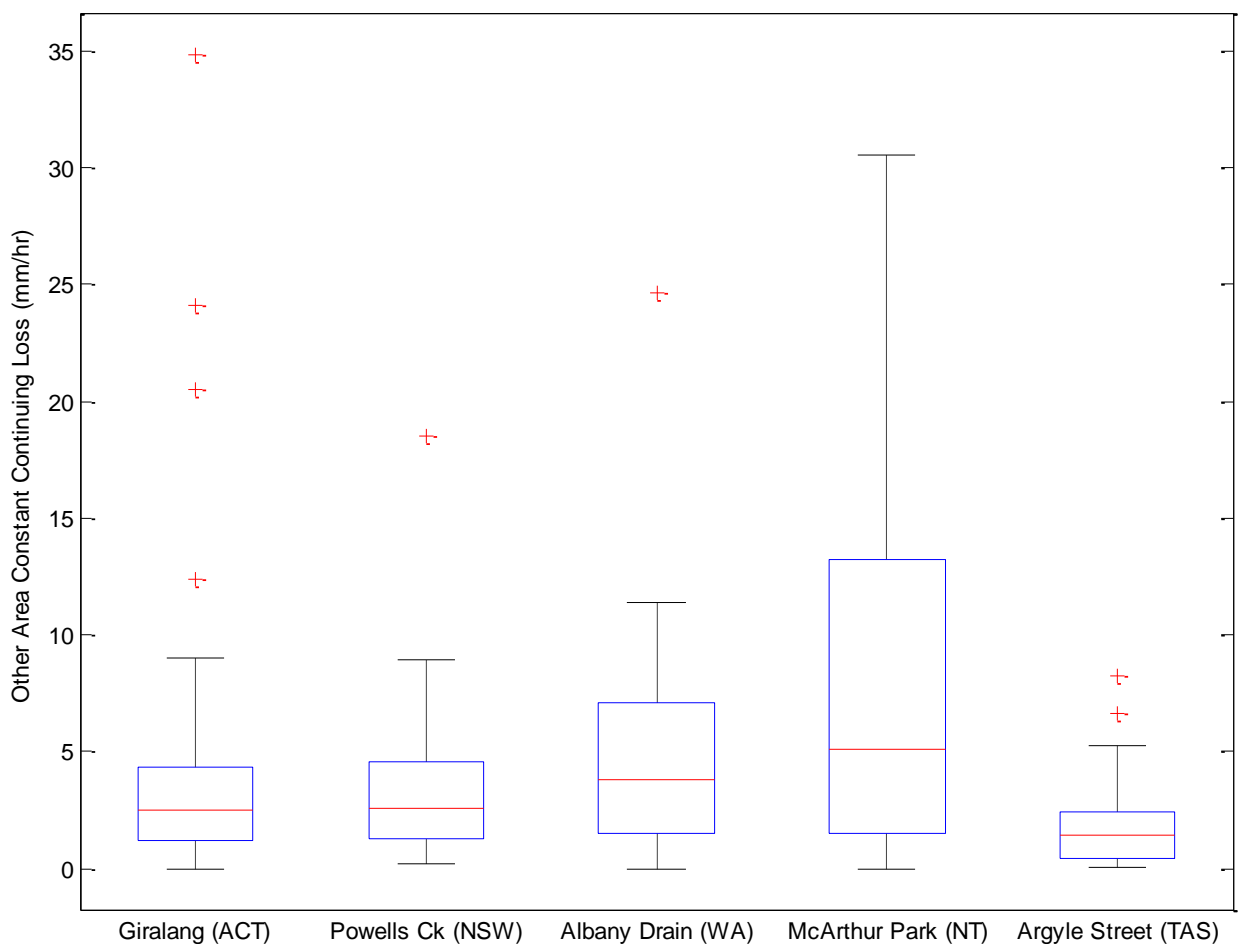
Figure ii. Other Area Constant Continuing Loss
