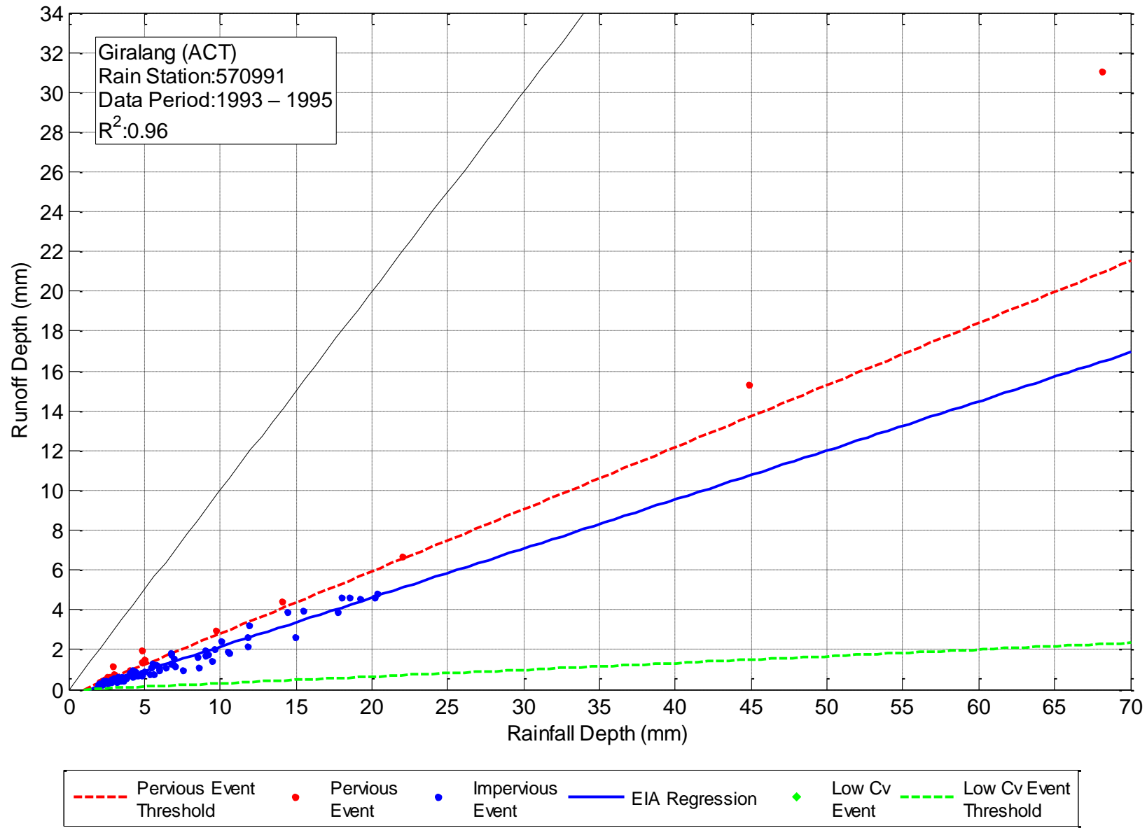
Figure C-6. Regression of Rainfall and Runoff – Giralang (ACT), Rain Gauge 570991, Data Period 1993 - 1995
