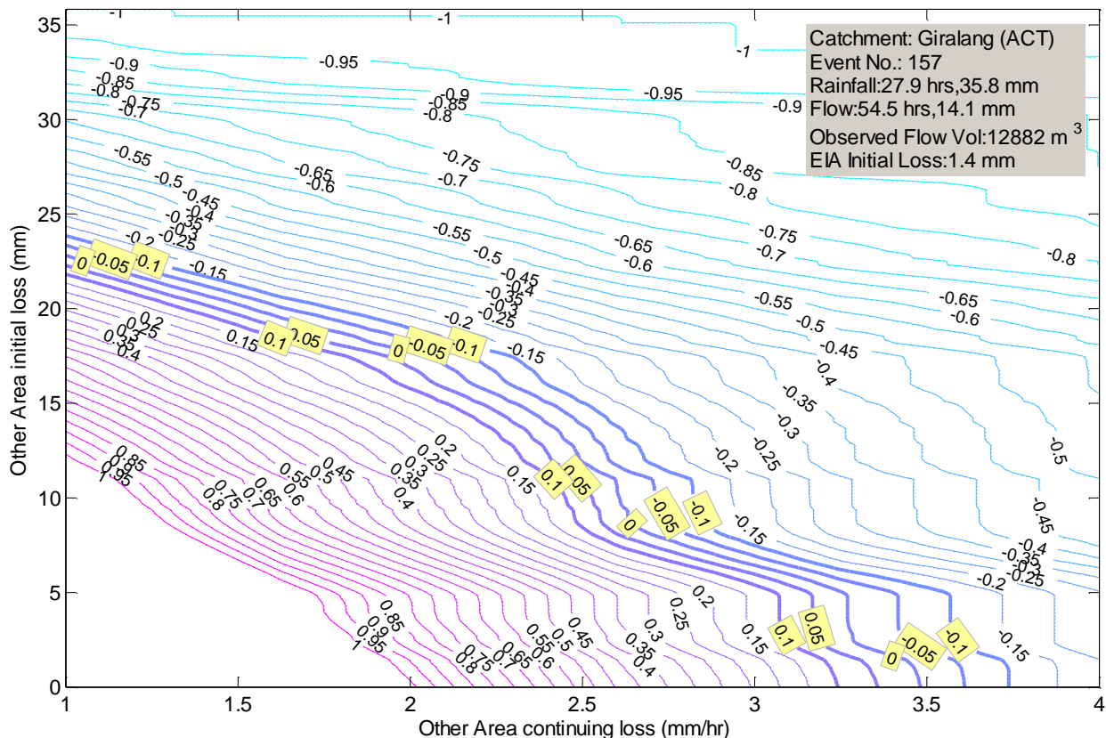
Figure 7-2 Error contours for different Initial Loss – Continuing Loss pairs for the Other Area. The Error is defined as (\text{Simulated Runoff Volume} - \text{Observed Runoff Volume}) / (\text{Observed Runoff Volume} - \text{EIA Runoff Volume}) .
