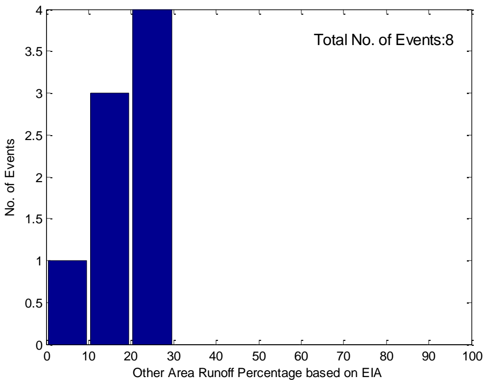
Figure 8-6. Parra Hills (SA) - Histogram of Identified Storm Events – Volume of Runoff from Other Area relative to total runoff
