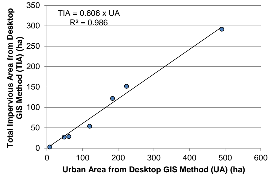
Figure 6-2 Relationships between Various Catchment Surface Variables
