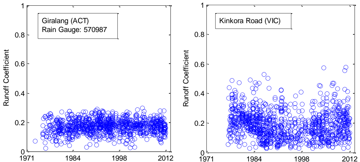
Figure 6-4 Variation of Runoff Coefficient with the recording period of the rainfall & streamflow data
