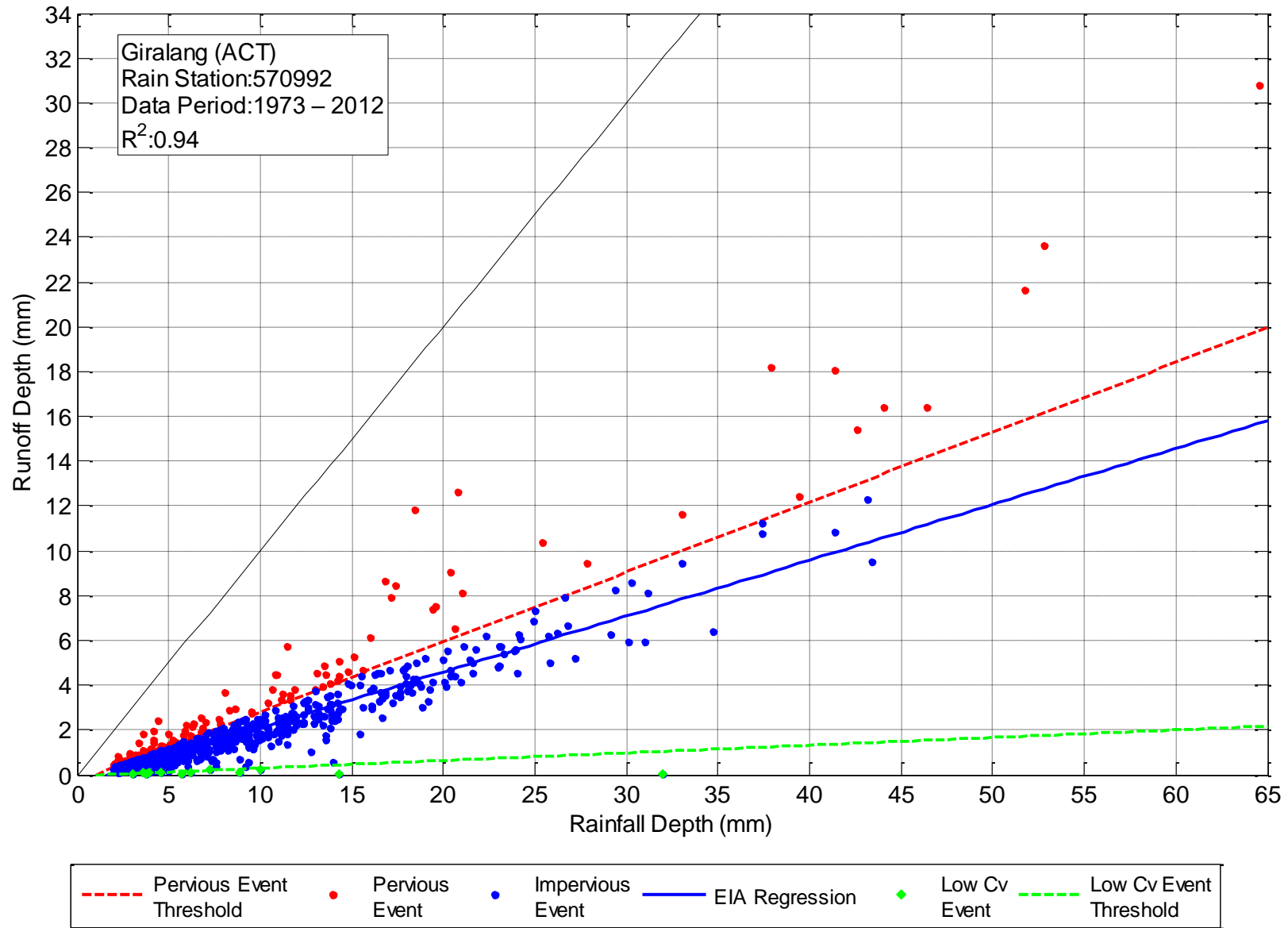
Figure C-8. Regression of Rainfall and Runoff – Giralang (ACT), Rain Gauge 570992, Data Period 1973 - 2012
