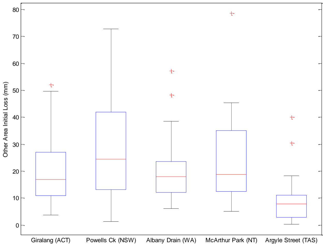
Figure i. Other Area Initial Loss Estimates
