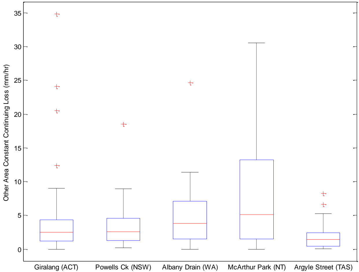
Figure 9-2 Boxplot of Other Area Constant Continuing Loss (Giralang: n = 41, Powells Ck: n = 14, Albany: n=30, McArthur Park: n = 20, Argyle Street: n = 49)
