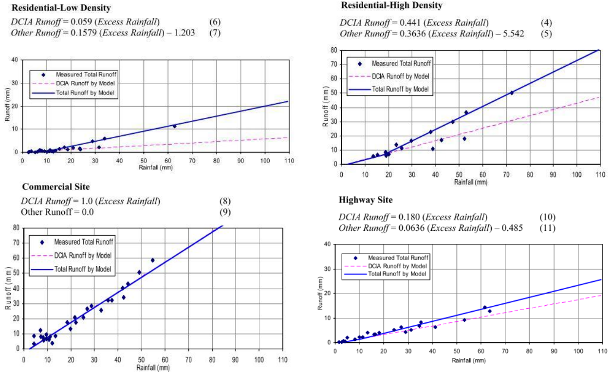
Figure 2-2 Rainfall – Runoff Relationship For Four Sites (Lee and Heaney, 2002)
